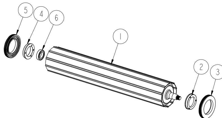
Roller, Special, ARC00168:
