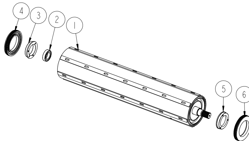
Roller, Large, ARC00034: QTY X 1.
